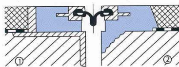
Expansion Joint B80B
